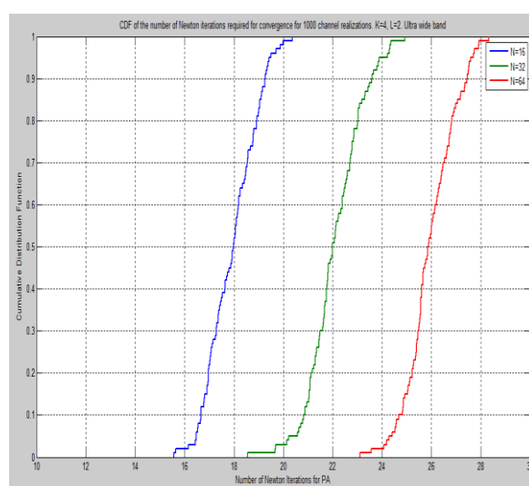
Fig.10 CDF of the number of newton iterations required for convergence for 1000 channel realization K=4, L=2 ultra wide band
