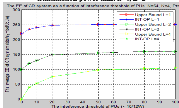
Fig.5 the EE of CR system as a function of interference threshold of Pus. N=64, k=4, Pt=1W
