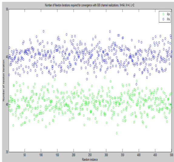
Fig.7 number of newton iterations required for convergence with 500 channel realizations. N=64, K=4, L
