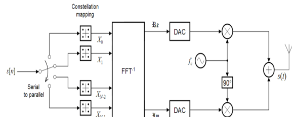
Fig.2 Transmitter
