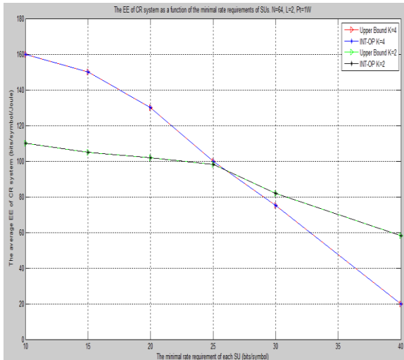
Fig.6 the EE of CR system as a function of the minimal rate requirements of SUs N=64, L=2, P_t=1W
