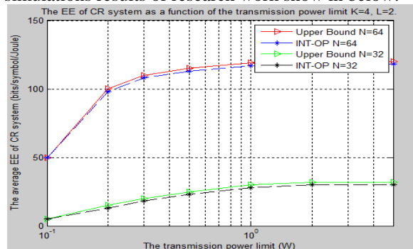
Fig.4 the EE of CR system as a function of the transmission power limit k=4, L=2
