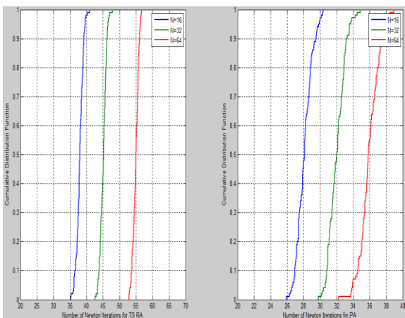
Fig.8 CDF of the number of Newton iterations required for convergence for 1000 channel realization K=4, L=2
