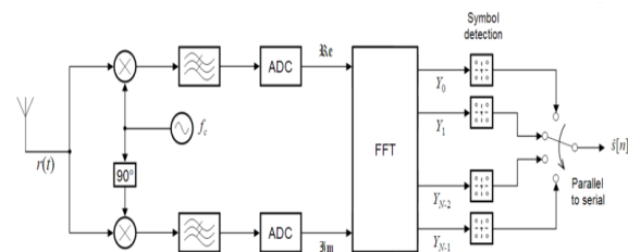
Fig.3 Receiver
