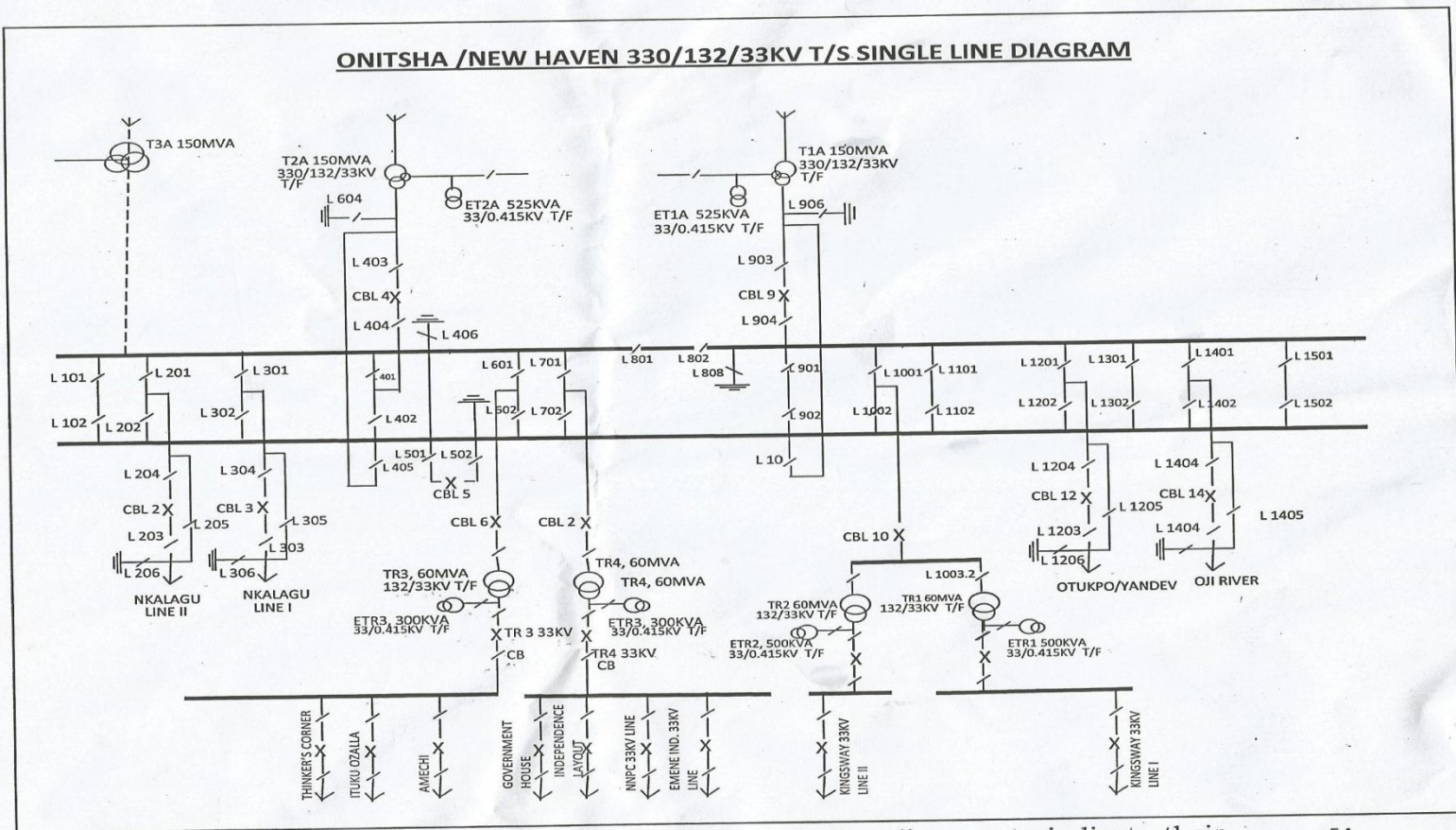
Fig. 4.1: Onitsha/New Haven 330/132/33KV single line diagram to indicate their stations.
