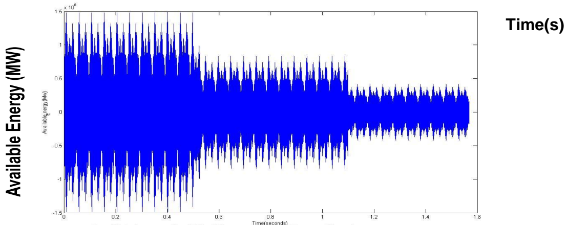
Figure 4.4: showing programmed step fall of available energy at 0.5 seconds, 0.8 seconds and 1.1 seconds
