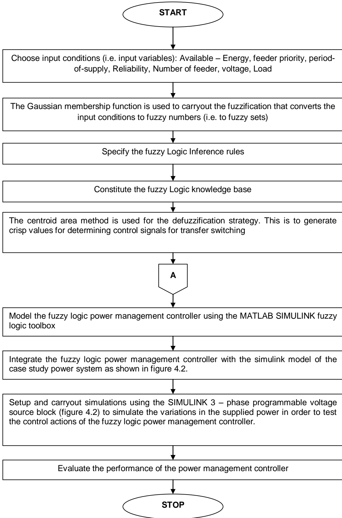
Flowchart for the fuzzy logic scheme
