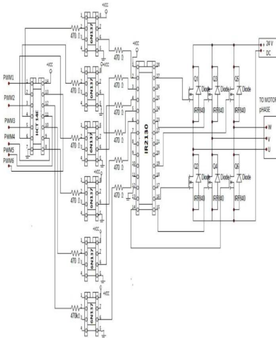
FIG: Circuit Diagram of STM32F407 Cortex M-4 Kit and Driver circuit
