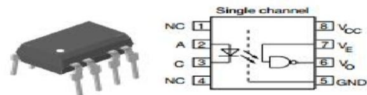
Figure 42: Pinout of 6N137 IC
