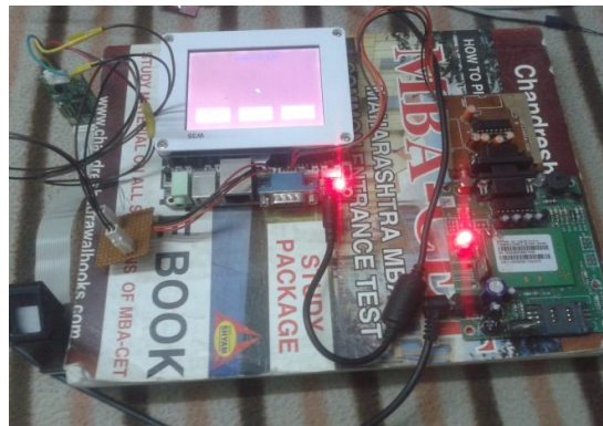
Figure.4: Photograph of completed prototype circuit
