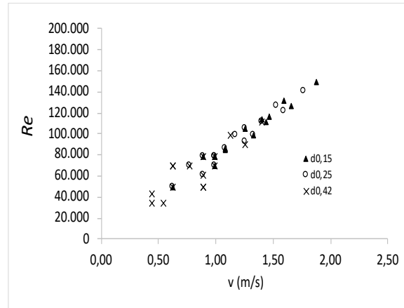
Figure 4. Relation between Re and V
