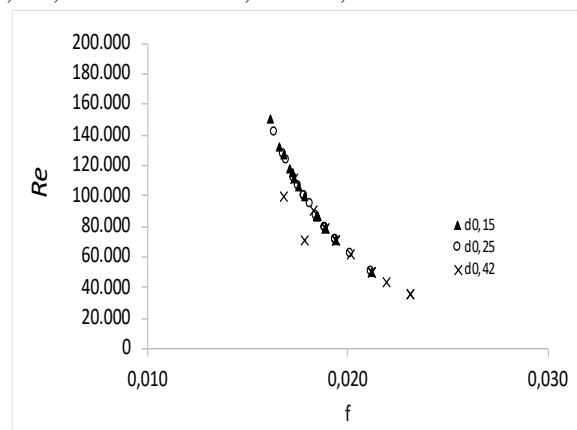
Figure 5. Relation between Re and f
