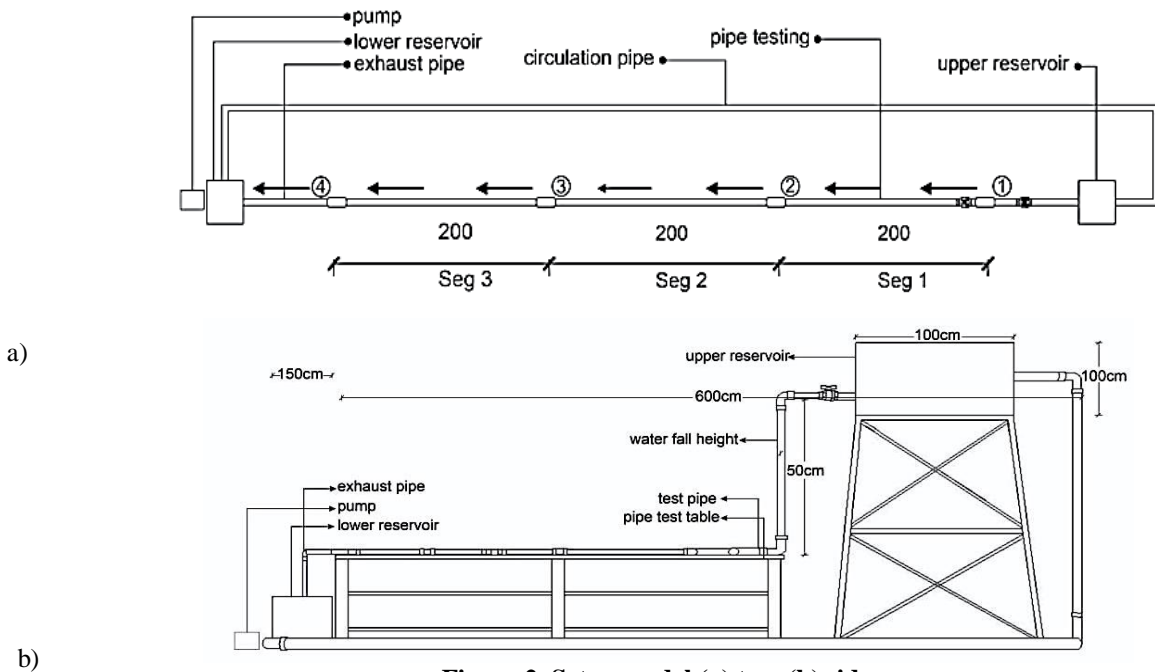
Figure 2. Setup model (a) top (b) side
