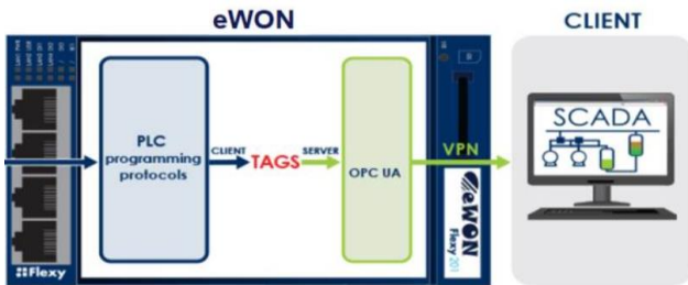
Fig 6: SCADA System
