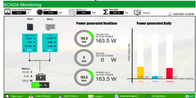
Fig 8: SCADA Monitoring
