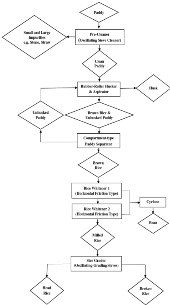
Fig 4: Flowchart of rice milling machine process
