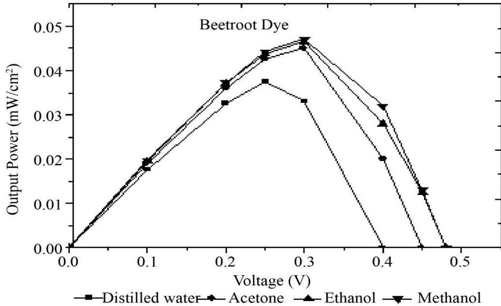
Fig. 10 Output power-voltage curves of DSSCs
