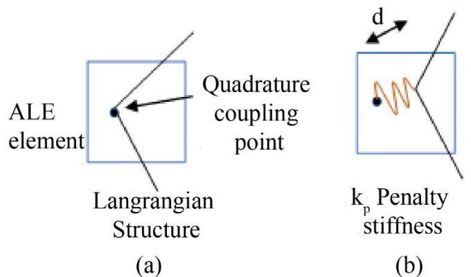
Fig. 2 Penalty coupling explained in (a), and (b)
